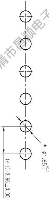
PCB HOLE LAYOUT
