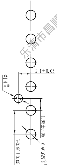
PCB HOLE LAYOUT
