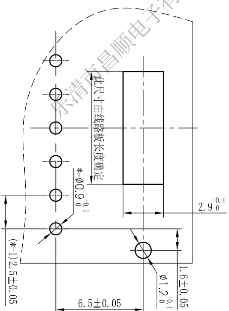
PCB HOLE LAYOUT
