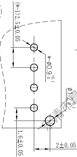
PCB HOLE LAYOUT
